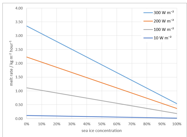
Figure 6: Melt rate against sea ice concentration for different solar radiation levels (Source: ESA CCI)
