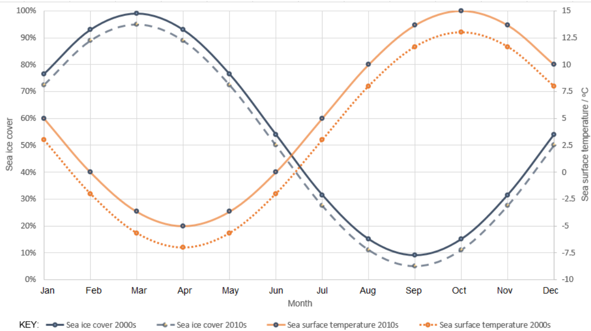
Figure 7: Seasonal cycles of sea ice extent and sea surface temperature (Source: ESA CCI)
