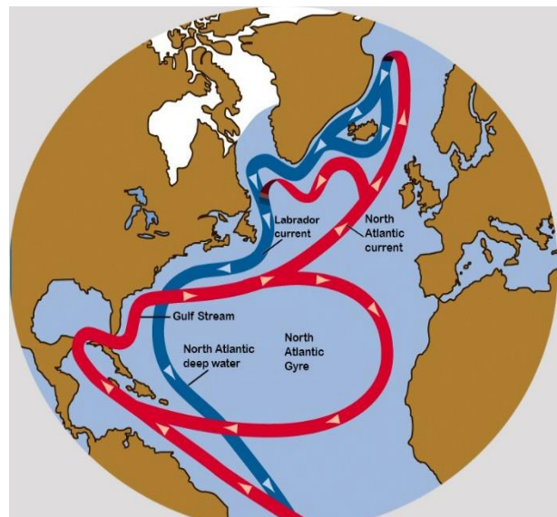
Figure 5: Oceanic thermohaline circulation in the Atlantic Ocean. Red lines indicate warm water, blue lines represent cold water and the arrowheads show the direction of the currents. (Source: ESA)
