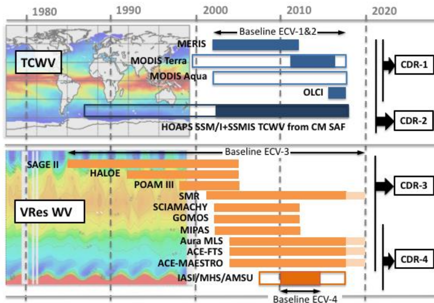
Figure 2-1: Instruments from which input observations (L2 data products) are obtained, and resulting climate data records (CDRs; L3 data products) for total column (TCWV; CDR-1 and CDR-2) and vertically resolved (VRes WV; CDR-3 and CDR-4) water vapour.
